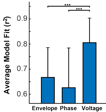
Figure 4: The instantaneous voltage of asymmetric oscillations is a better predictor of cortical excitability than either oscillatory power or phase. Y-axis gives average model fits ( r^2 s) for each of the three cases. Bars give the median model fit with error bars representing the 75th percentile. *** p < 0.001 , paired Wilcoxon Signed Rank test.
