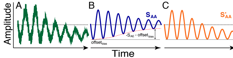
Figure 2: Extraction of the instantaneous voltage. (A) gives the time course of a simulated rhythmic signal contaminated by non-rhythmic noise. (B) gives the result of band-pass filtering the signal shown in (A). This procedure removed noise, but also removed the bias in the data and made the signal zero-mean. (C) shows the result after adding the bias back into the data. Troughs are at the same amplitude throughout.
