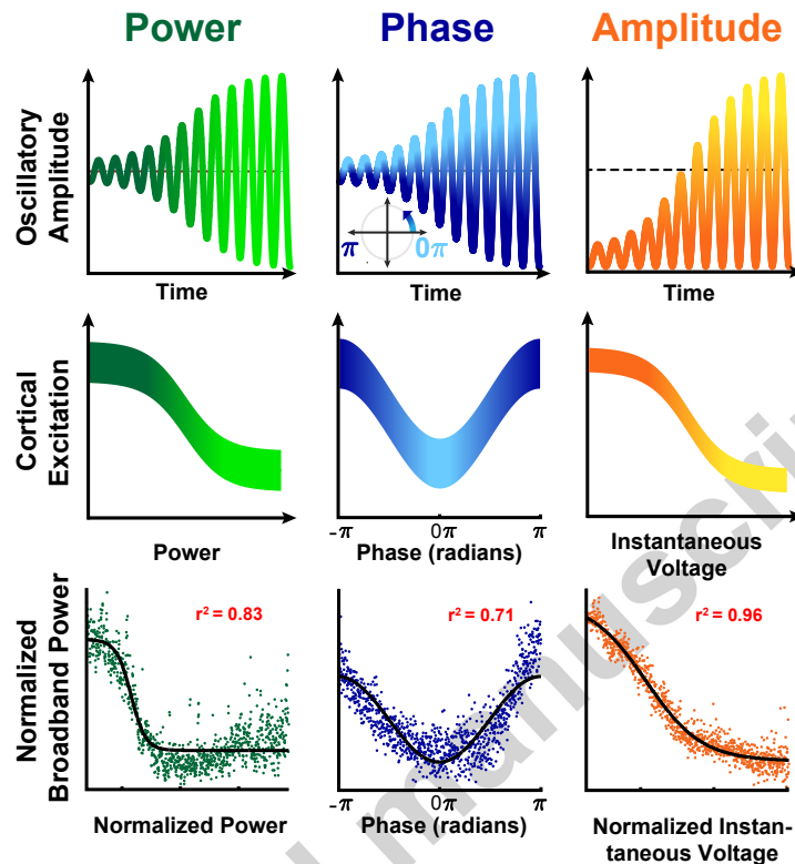
Figure 1: Comparison of the three measurements of oscillatory power, phase, and instantaneous amplitude, their relationship to cortical excitation, and exemplary experimental data from one location. Top row: Left and center panels show exemplary waveforms of band-pass filtered oscillatory activity with zero mean as implied by traditional measurements of oscillatory power and phase, respectively. Right panel shows exemplary waveforms of asymmetric oscillatory activity as proposed by the FBO hypothesis. Y axes give signal amplitude; X axes give time. Color gradients indicate each measurement's theoretical relationship to cortical excitability: darker colors correspond to high excitability, and light colors correspond to low excitability. E.g., the left part of the green trace has low oscillatory power and is associated with high cortical excitability as indicated by the dark green color. Middle Row: Each measurement's relationship with cortical excitation (y-axis). Color gradients correspond to those in the top row. Left panel: cortical excitability (dark green color) and resulting excitation (value on y-axis) are high when oscillatory power is low. Center panel: cortical excitation and excitability are high when the oscillation is at its trough (i.e., \pm\pi ). Right panel: cortical excitation and excitability are high when the instantaneous voltage is low. Bottom Row: Exemplary experimental data from one ECoG location. Each dot gives the average normalized broadband power within one of 1000 bins that are spaced linearly across each of the three X axes. These data, and their parametric fits using sigmoid/cosine functions, conform to expectations illustrated in the middle row. X-axes give normalized broadband activity (an index of cortical excitation and a proxy for cortical excitability). In this exemplary channel, the fit (assessed as r^2 ) of the model to the data is 0.83 for power, 0.71 for phase, and 0.96 for instantaneous voltage.
